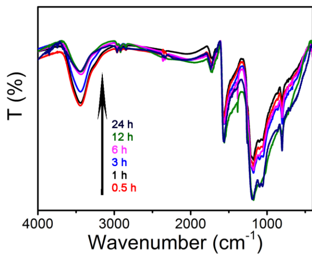
Fig. S1 FTIR spectra of GO reduced by OA and NaI for different duration.
